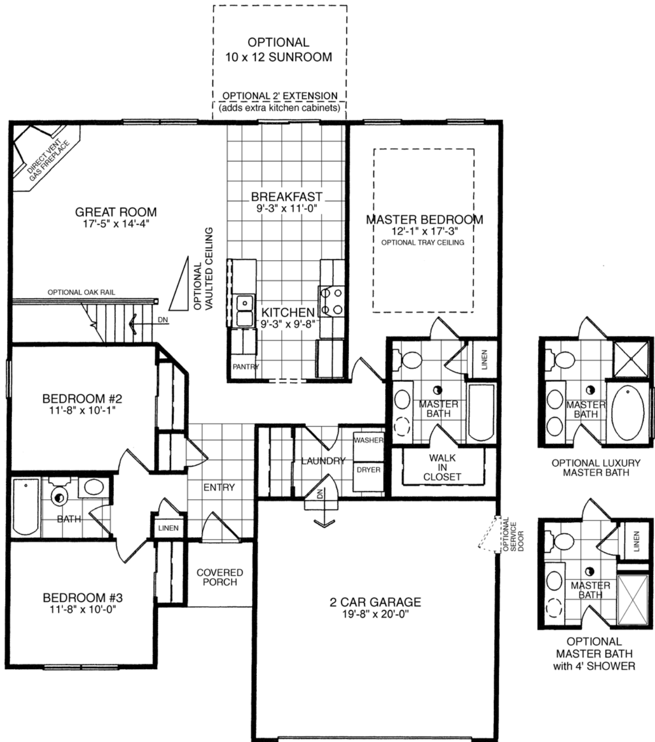
First Floor Plan - Elevation A
