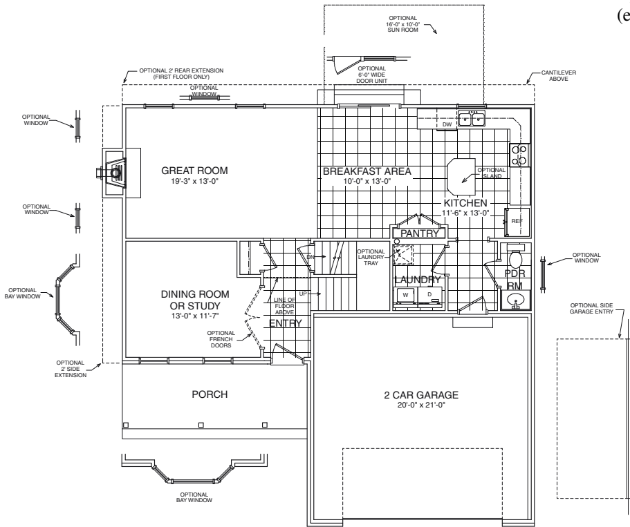
First Floor Plan Elevation C
