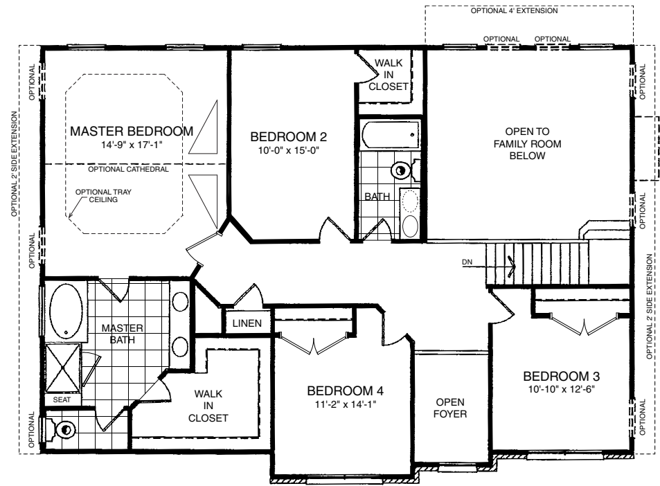
SECOND FLOOR PLAN - ELEVATION A
