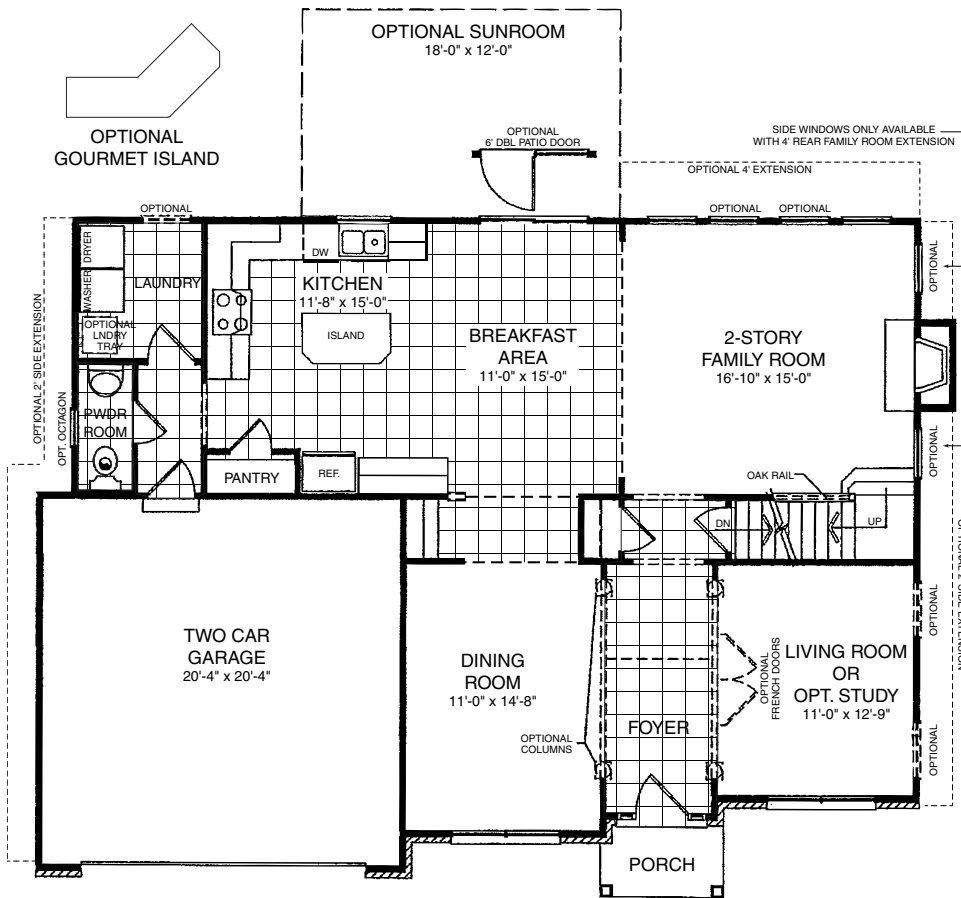
FIRST FLOOR PLAN - ELEVATION A
